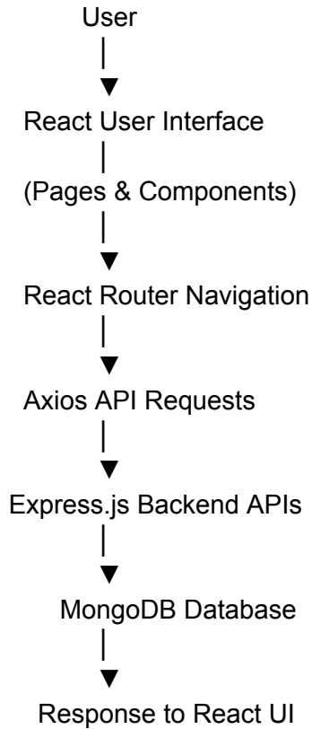
Figure 1: Frontend Workflow
